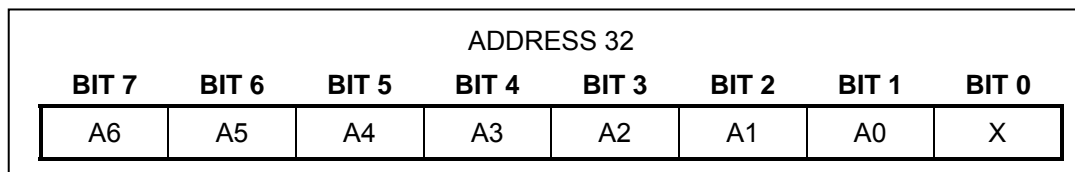
Figure 15. Slave Address Format
