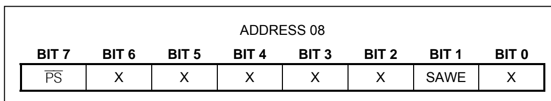
Figure 14. Special Feature Register Format
