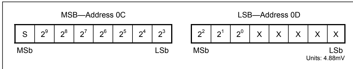
Figure 8. Voltage Register Format
