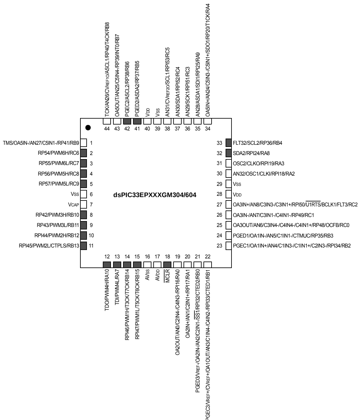
44-Pin QFN (1,2,3)
