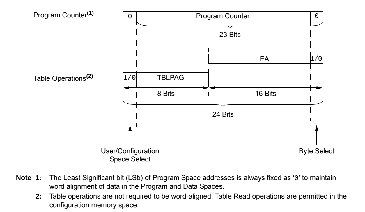
FIGURE 4-16: DATA ACCESS FROM PROGRAM SPACE ADDRESS GENERATION
