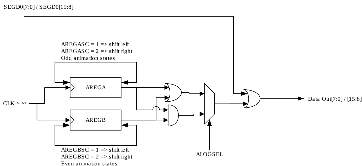
Figure 33.44. LCD Block Diagram of the Animation Circuit
