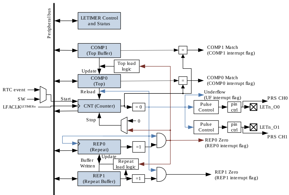
Figure 23.1. LETIMER Overview
