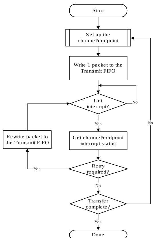
Figure 15.8. Transmit Transaction-Level Operation in Slave Mode
