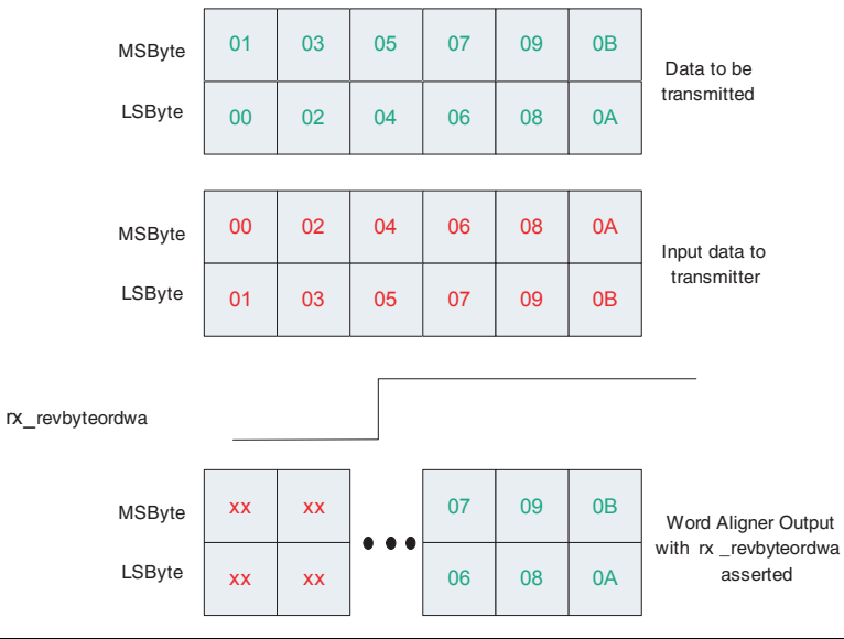
Figure 2–71. Receiver Byte Reversal Feature
