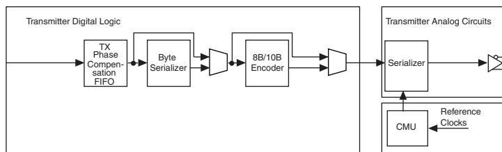
Figure 1–2. Stratix II GX Transmitter Block Diagram
