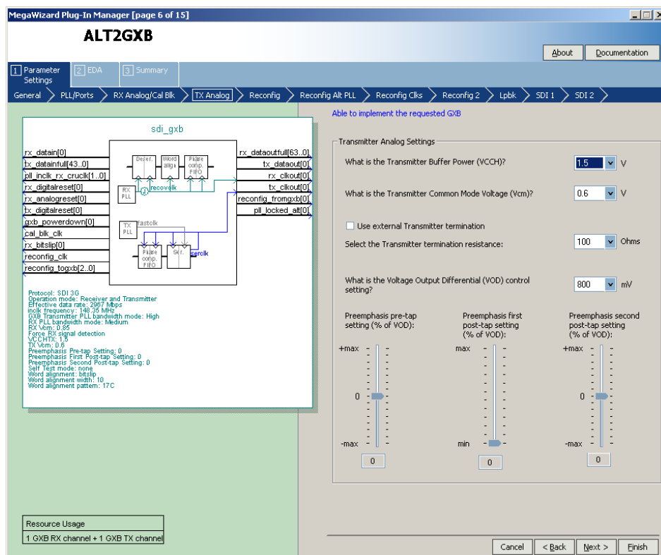
Figure 4–87. MegaWizard Plug-In Manager - ALT2GX (TX Analog)
