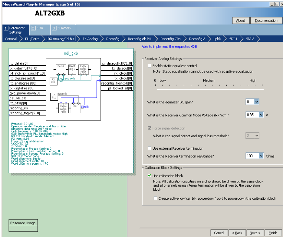
Figure 4–86. MegaWizard Plug-In Manager - ALT2GXB (RX Analog/Cal Blk)
