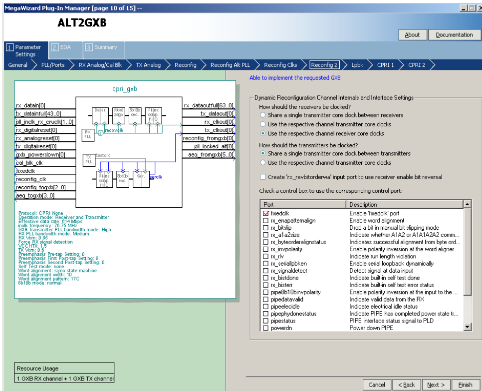
Figure 4-78. MegaWizard Plug-In Manager - ALT2GXB (Reconfig 2)
