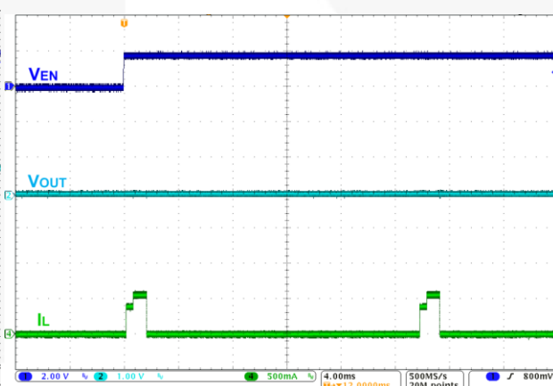
Figure 20. Fault Restart
