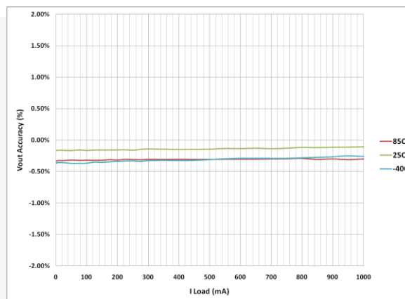
Figure 12. Output Regulation vs. Load Current and Temperature
