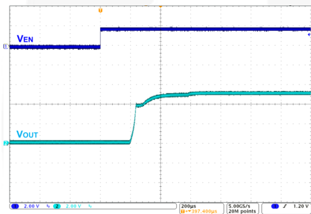
Figure 19. Startup, 150 mA Load
