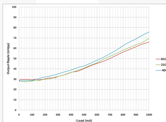
Figure 14. Output Ripple vs. Load Current and Temperature
