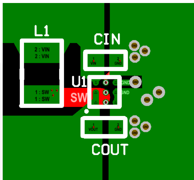
Figure 22. Layout Recommendation
