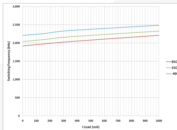
Figure 10. Switching Frequency vs. Load Current and Temperature
