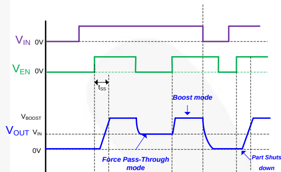
Figure 21. Pass-Through Profile
