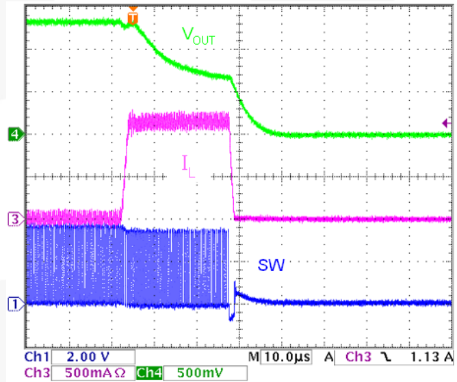
Figure 32. R_{LOAD} = 660 mΩ
