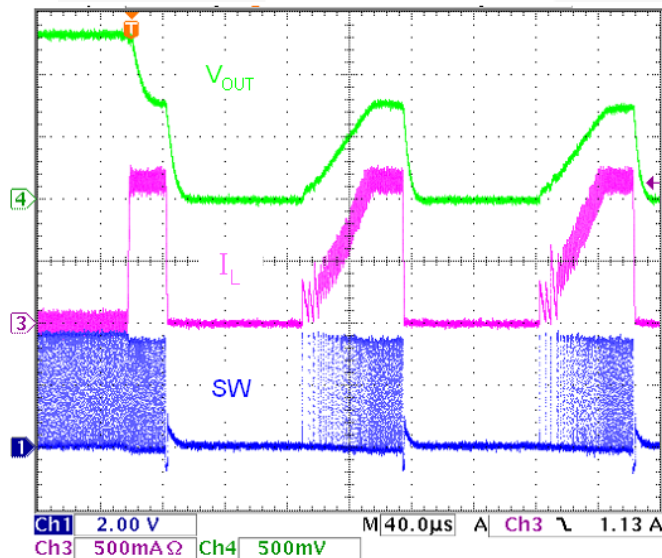
Figure 31. R_{LOAD} = 660 mΩ
