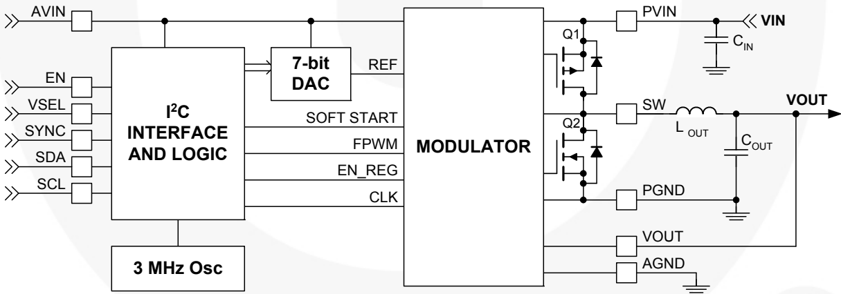
Figure 4. Block Diagram
