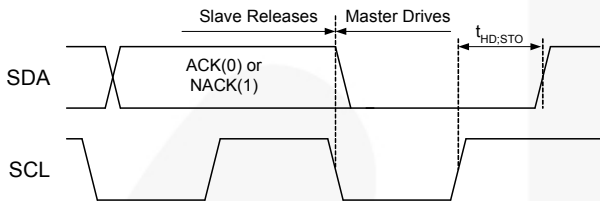
Figure 43. Stop Bit
