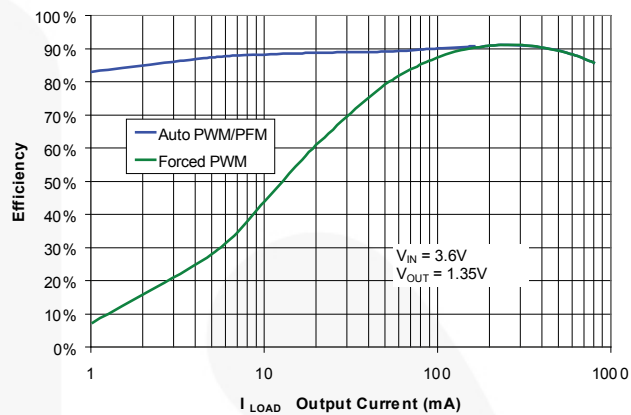
Figure 8. Efficiency vs. Load at V_{OUT} = 1.35\text{ V}
