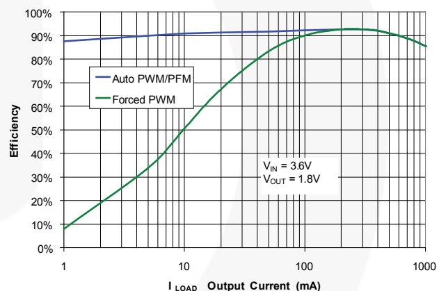
Figure 10. Efficiency vs. Load at V_{OUT} = 1.80\text{ V}
