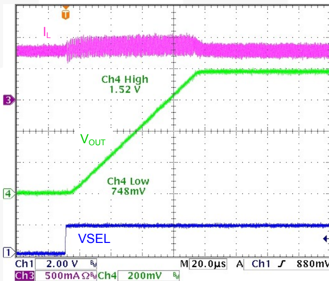
Figure 28. Multi-Step, Controlled DAC Step (9.6 mV/ \mu\text{s} ) DEF_Slew 6 (110), 800 mA Load
