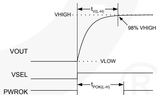
Figure 39. Single-Step V_{OUT} Transition
