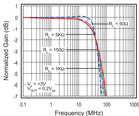
Figure 8. Frequency Response vs. R_L (+3V)
