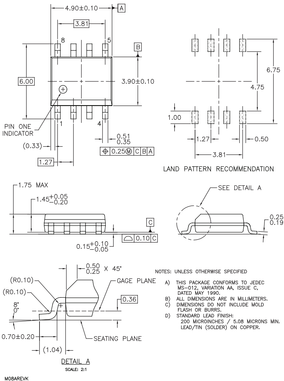
Figure 47. SOIC-8 Package
