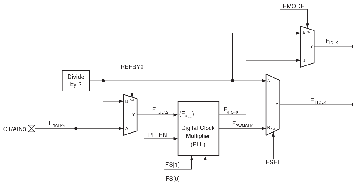
Figure 4. External Clock Scheme
