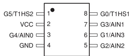
FMS7401L 8-Pin TSSOP
