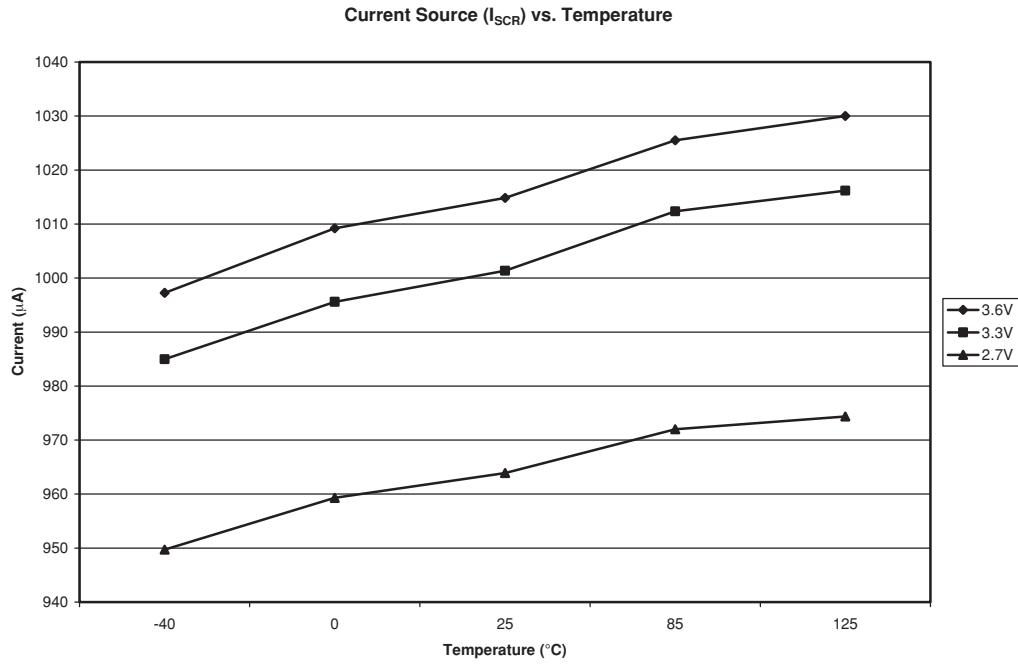
Figure 36. Current Source ( I_{SCR} ) vs. Temperature
