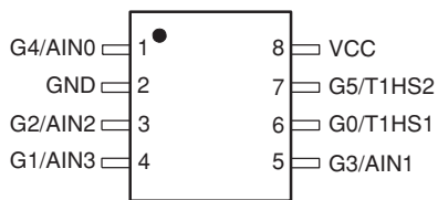
FMS7401L 8-Pin PDIP/SOIC
