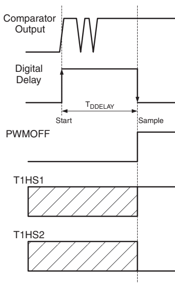
Figure 10. Digital Delay Timing
