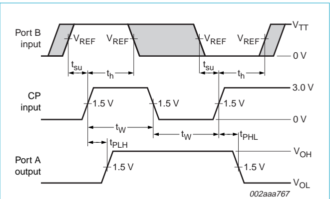
Fig 5. CP to A timing.
