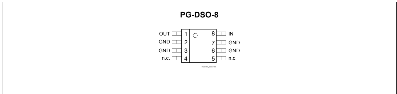
Figure 2 Pin Configuration
