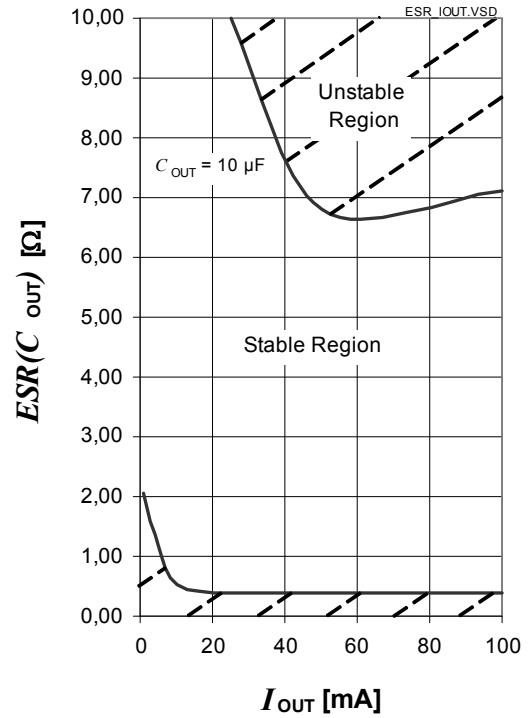
IFX2931GV50: Output Capacitor's Equivalent Series Resistance ESR(C_{OUT}) versus Output Current I_{OUT}
