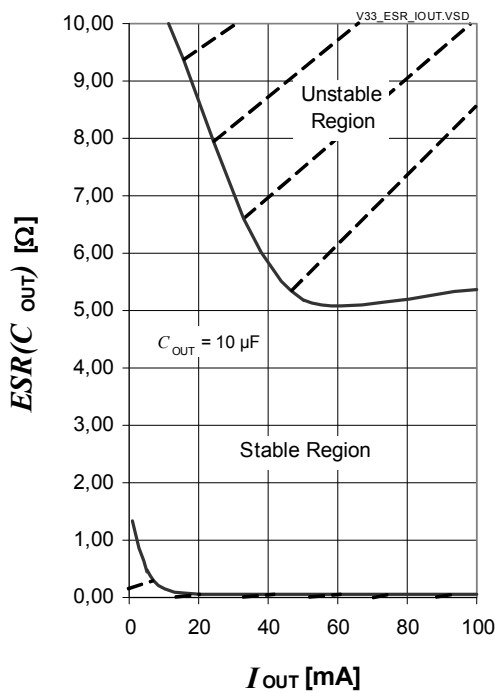
IFX2931GV33: Output Capacitor's Equivalent Series Resistance ESR(C_{OUT}) versus Output Current I_{OUT}
