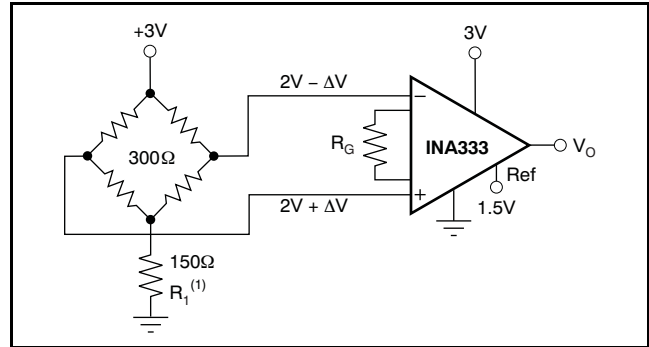
Figure 37. Single-Supply Bridge Amplifier
