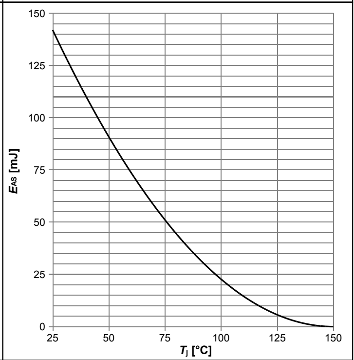
Diagram 16: Avalanche energy
