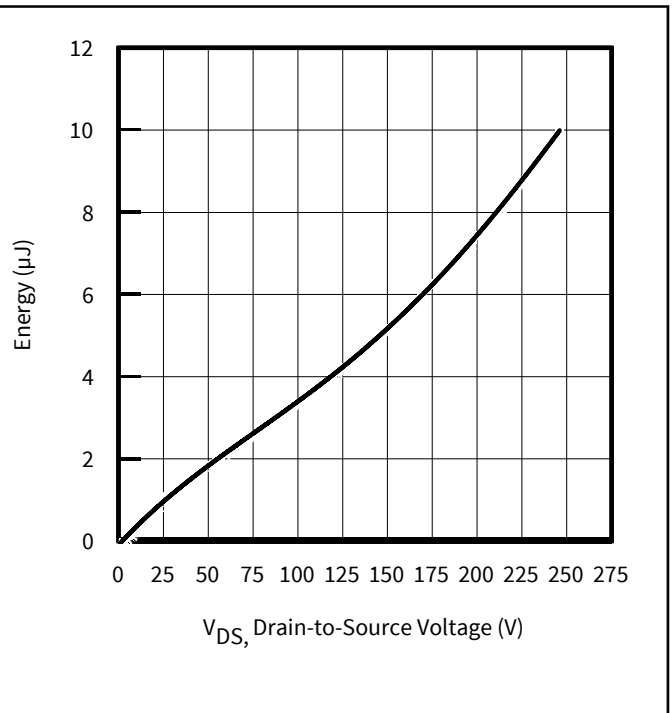
Figure 12 Typical Coss Stored Energy
