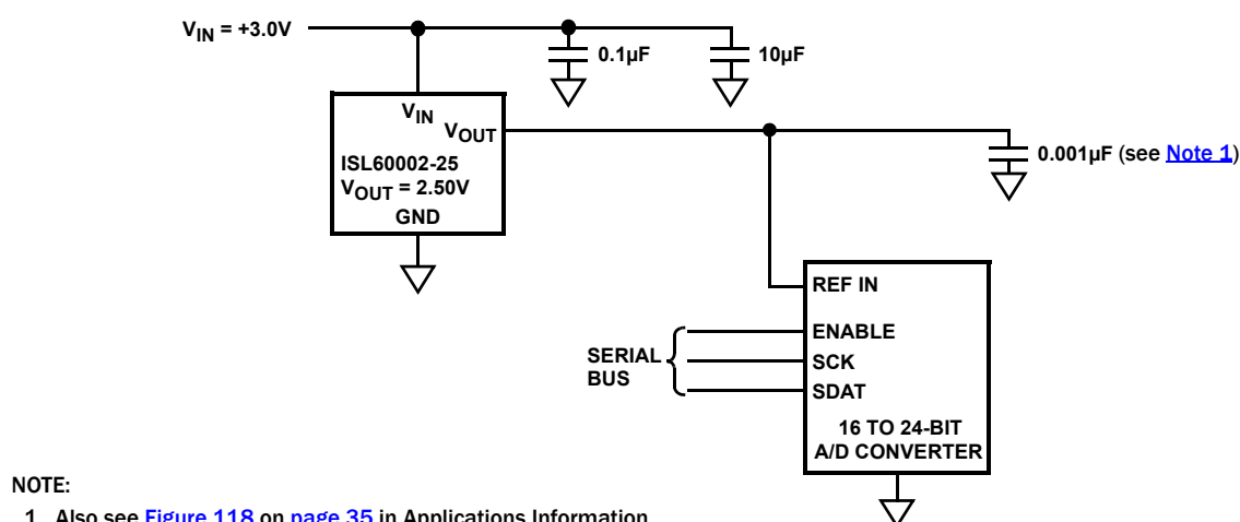
FIGURE 1. TYPICAL APPLICATION
