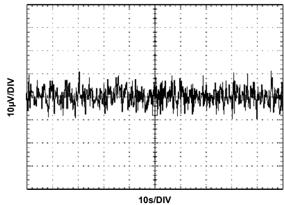
FIGURE 41. V_{OUT} NOISE
