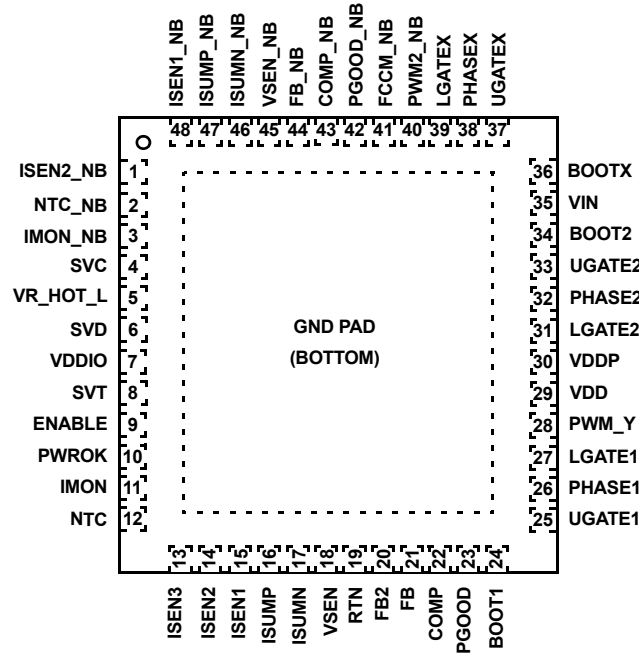
ISL6277A (48 LD QFN) TOP VIEW
