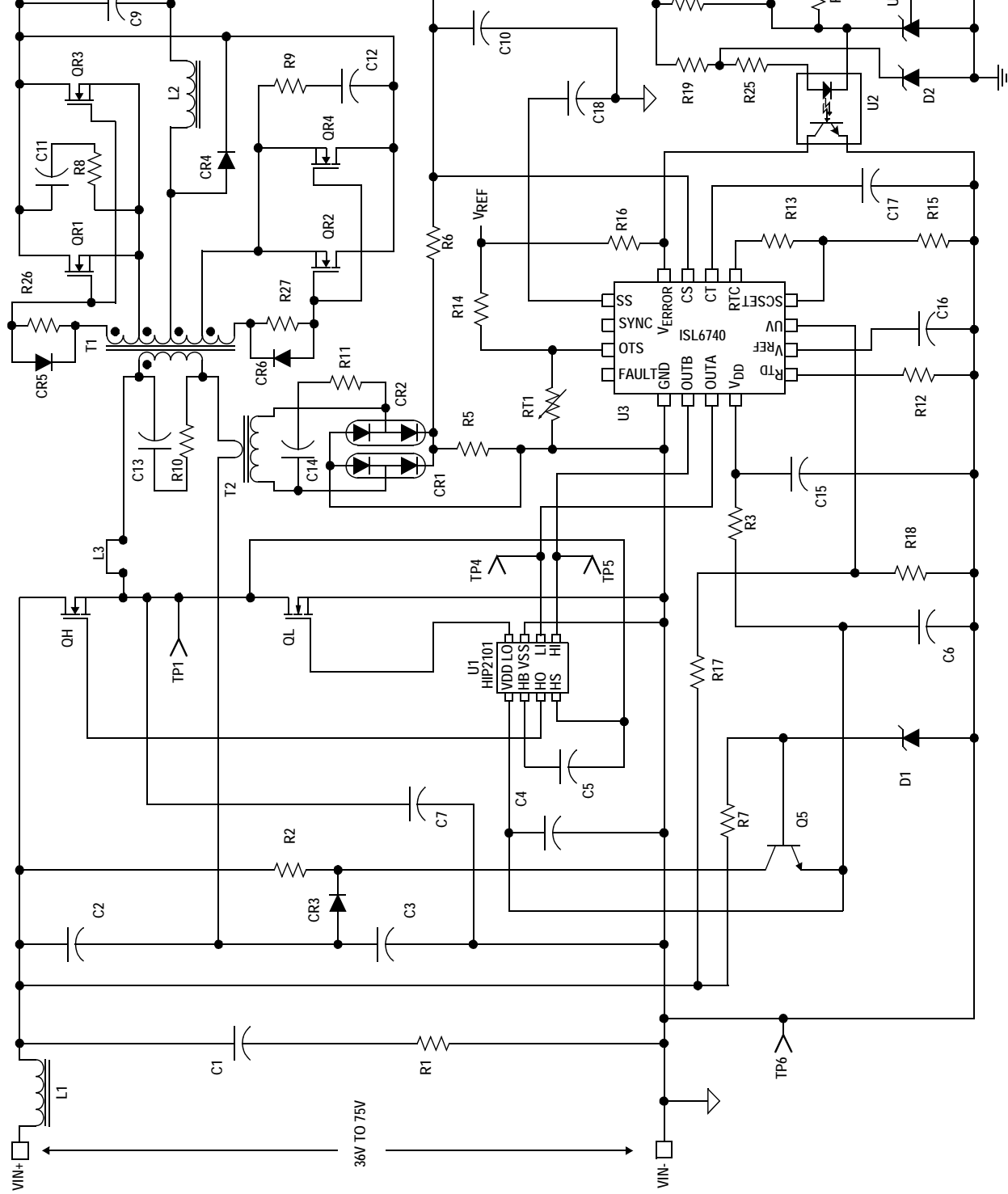
FIGURE 4. TYPICAL APPLICATION (ISL6740EVAL2Z)
