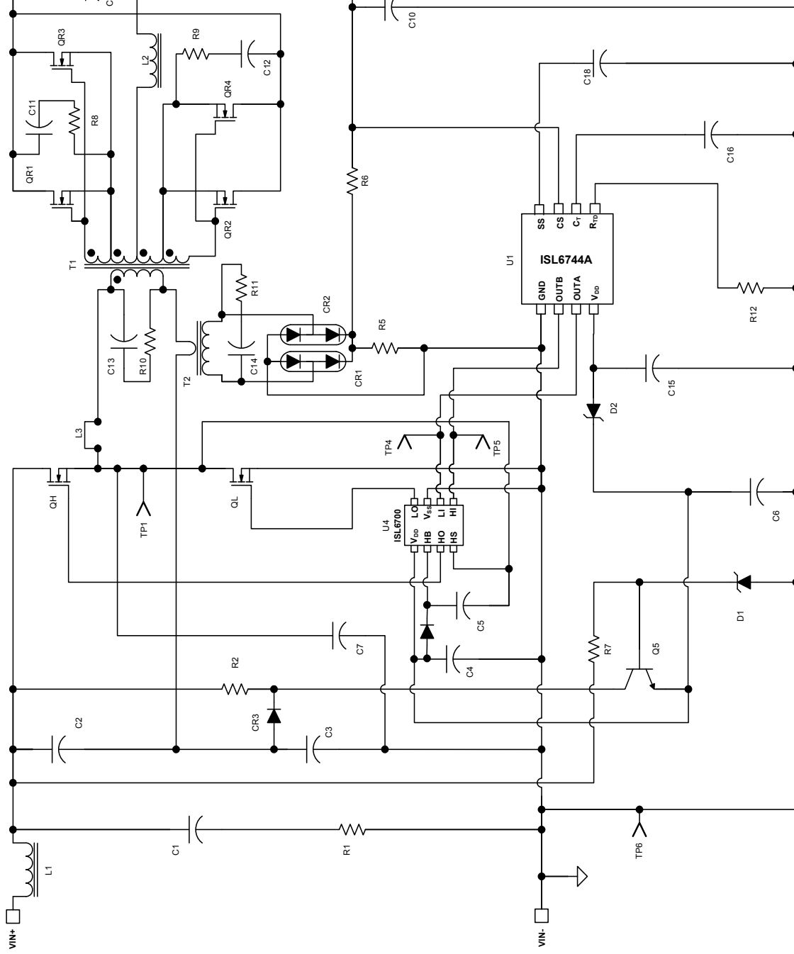
Figure 2. Typical Application Using ISL6744A - 48V Input DC Transformer, 12V at 8A Output
