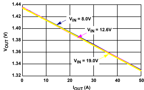
FIGURE 10. NOMINAL MODE DROOP IMPEDANCE, 2 PHASE, CCM, LP = HIGH, VSEL = 1.435V
