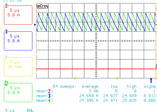
FIGURE 18. 2 PHASE CURRENT BALANCE, FULL LOAD = 50A
