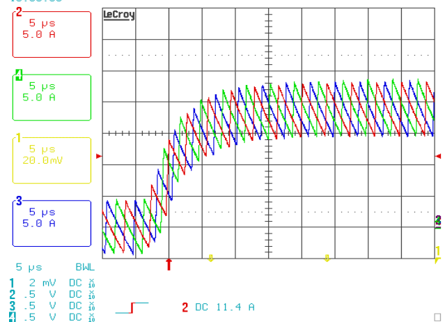
FIGURE 21. TRANSIENT LOAD 3 PHASE OPERATION, ZOOM OF RISING EDGE CURRENT BALANCE
