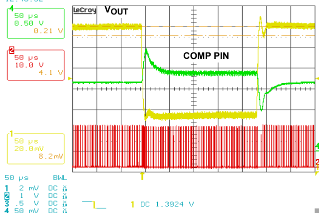
FIGURE 19. TRANSIENT LOAD RESPONSE, 40A LOAD STEP @ 200A/μs, 3 PHASE
