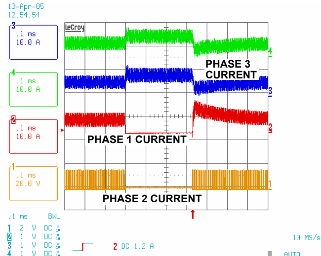
FIGURE 33. ISL9506, INDUCTOR CURRENT WAVEFORM WITH PHASE ADDING AND DROPPING IN CCM OR NOMINAL MODE
