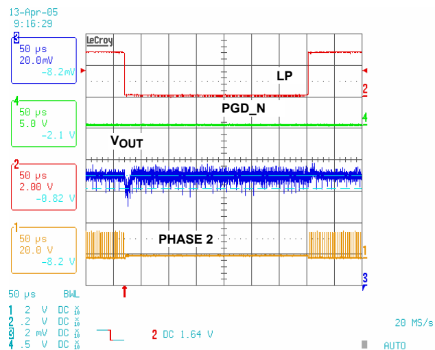
FIGURE 30. ISL9506, PHASE ADDING AND DROPPING IN NOMINAL MODE, LOAD CURRENT = 15A
