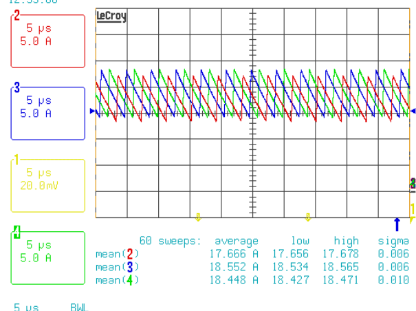
FIGURE 17. 3 PHASE CURRENT BALANCE, FULL LOAD = 50A
