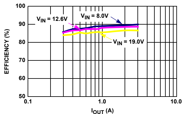
FIGURE 8. DIODE EMULATION MODE EFFICIENCY, 2 PHASE, DCM OPERATION, LP = LOW, VSEL = 1.4375V
