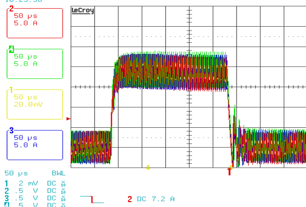
FIGURE 20. TRANSIENT LOAD 3 PHASE OPERATION - CURRENT BALANCE
