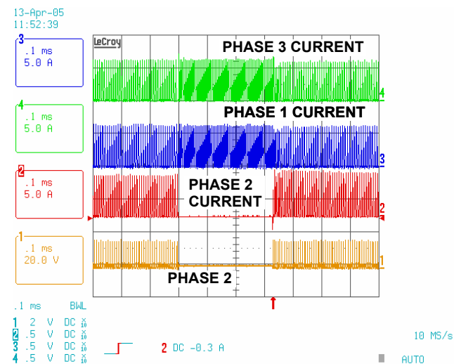
FIGURE 32. ISL9506, INDUCTOR CURRENT WAVEFORM WITH PHASE ADDING AND DROPPING IN DCM OR DIODE EMULATION MODE
