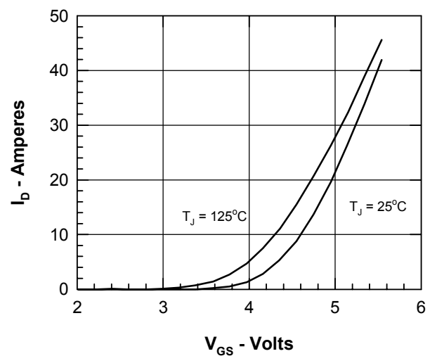
Figure 6. Admittance Curves
