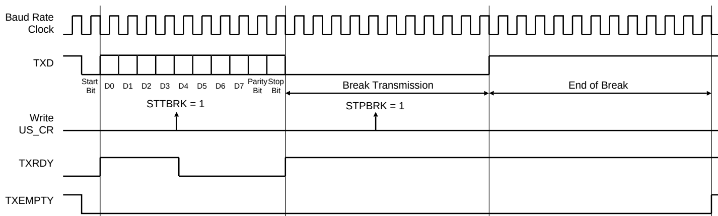
Figure 34-26. Break Transmission
