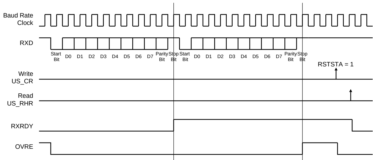
Figure 34-21. Receiver Status
