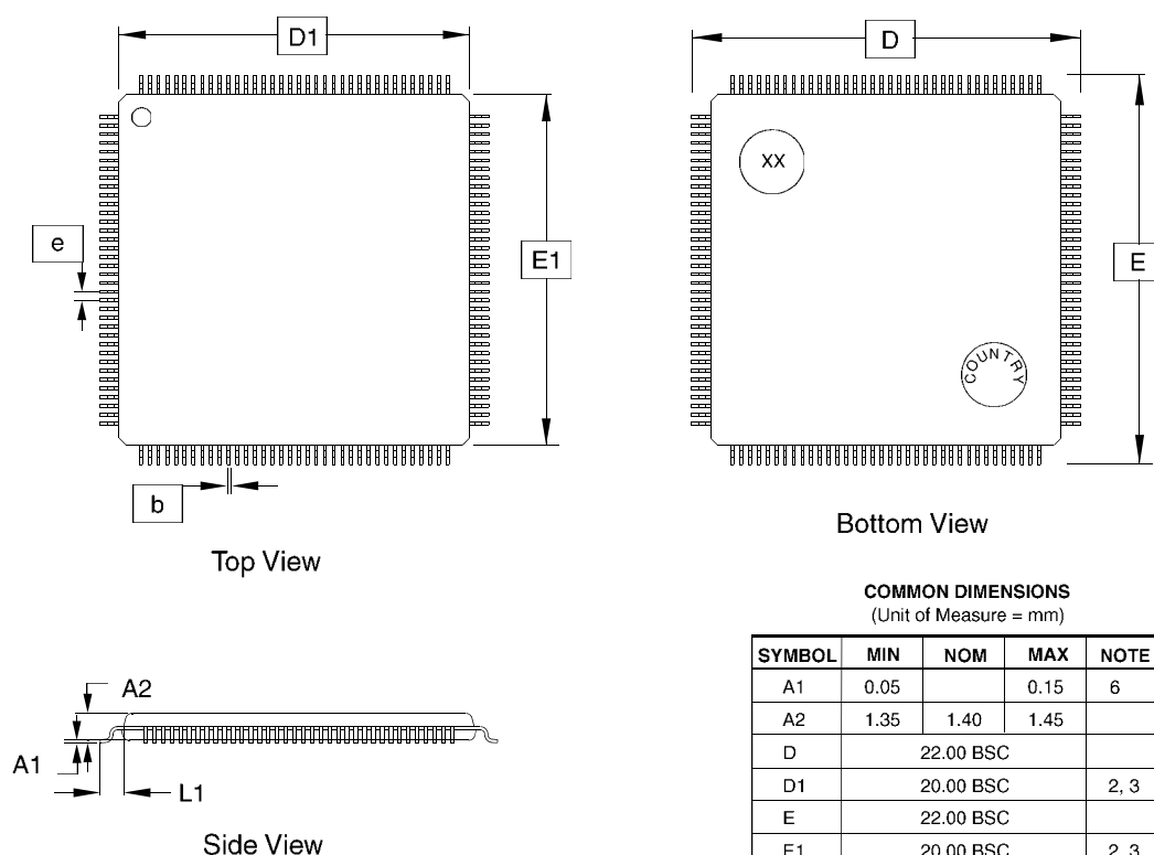
Figure 43-3. 144-lead LQFP Package Drawing
