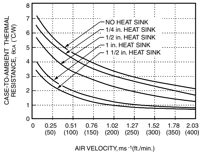
Figure 35. Case-to-Ambient Thermal Resistance vs. Air Velocity Curves; Either Orientation
