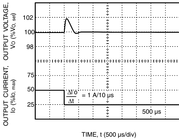
Figure 17. JW030D-M, F-M, G-M Typical Output Voltage for a Step Load Change from 50% to 25%
