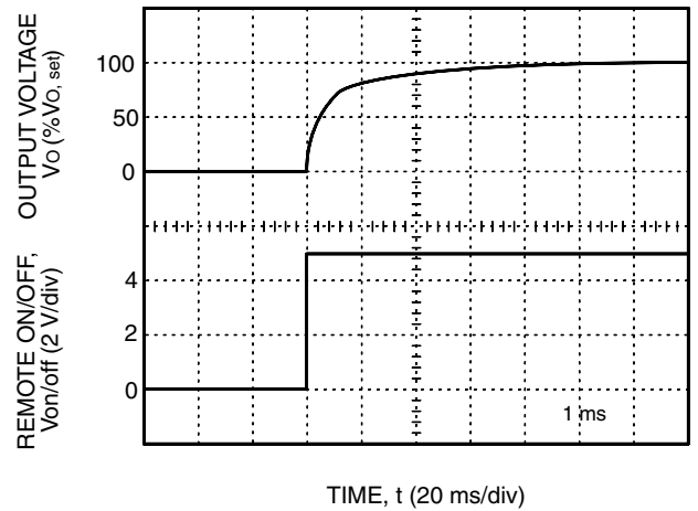
Figure 19. Typical Output Voltage Start-Up when Signal Applied to Remote On/Off
