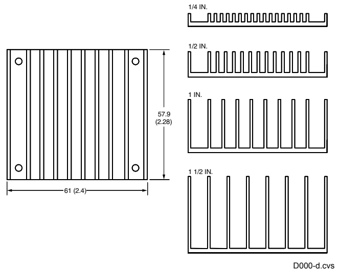
Figure 37. Transverse Heat Sink
