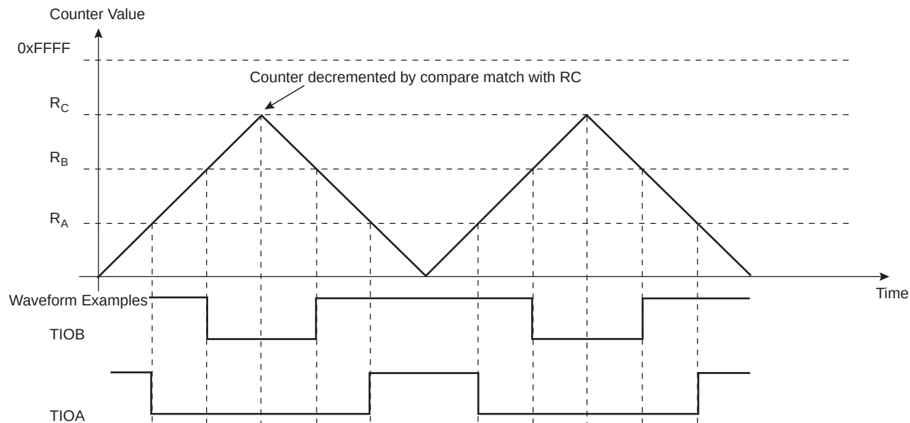
Figure 47-14.WAVSEL = 11 without Trigger
