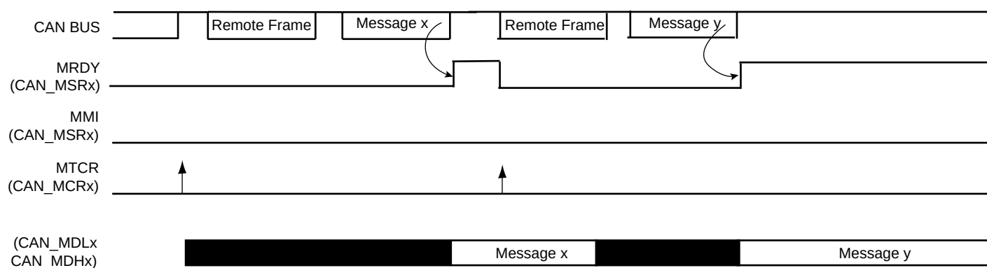
Figure 45-18.Consumer Handling
