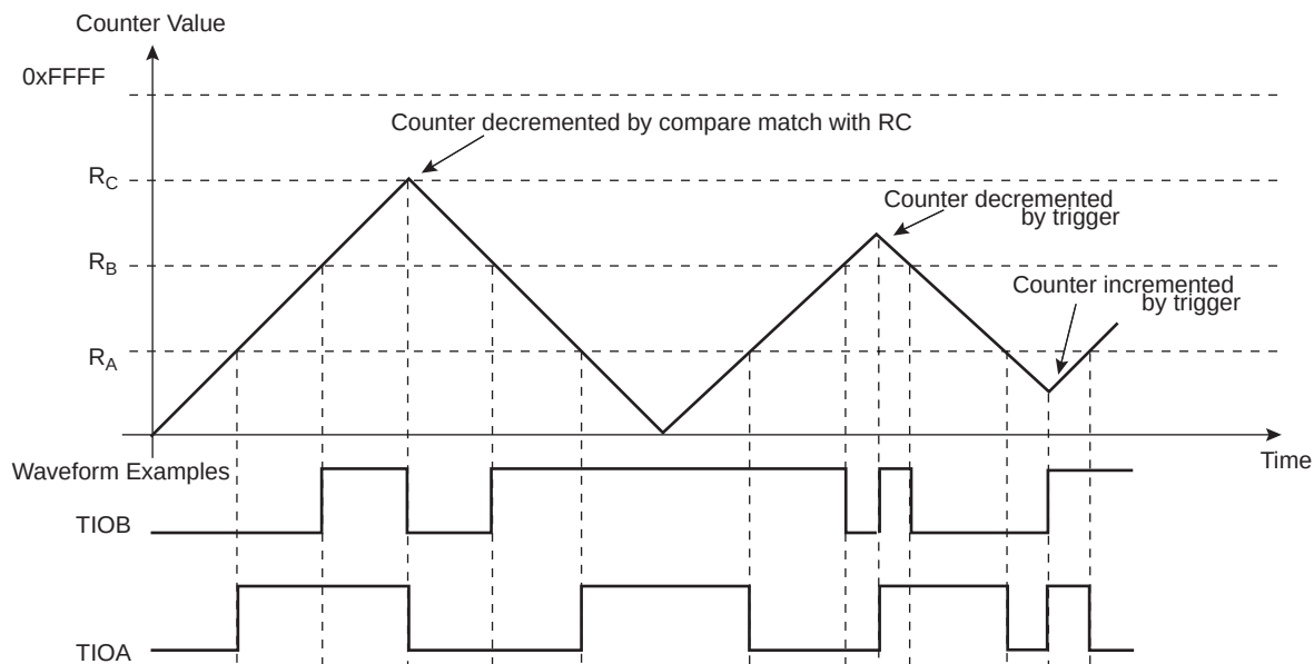
Figure 47-15.WAVSEL = 11 with Trigger
