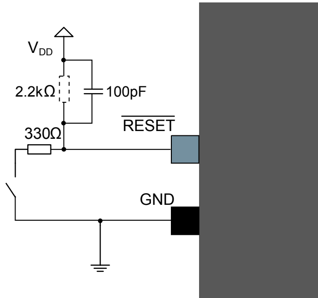
Figure 35-4. External Reset Circuit Schematic
