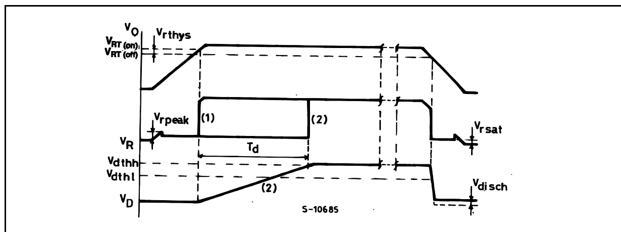
Figure 2: Reset Waveforms:
