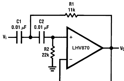
Figure 60. Sine Wave Oscillator
