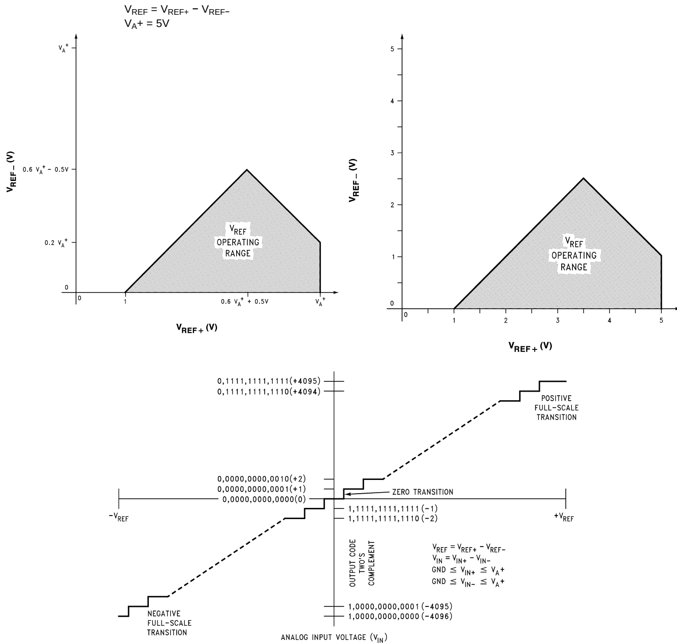
Figure 4. Transfer Characteristic
