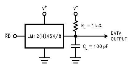
Figure 40. TRI-STATE Test Circuits and Waveforms
