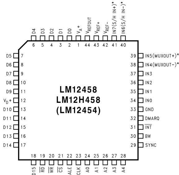
Figure 1. See Package Number FN0044A
