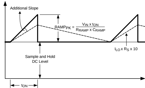
Figure 20. Composition of Emulated Current Sense Signal
