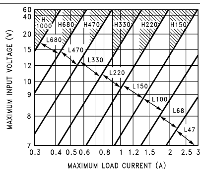
Figure 28. LM2576(HV)-5.0
