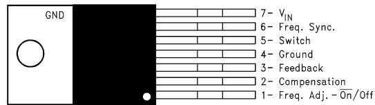
NDZ Package 7-Pin TO-220 Top View, Bent, Staggered Leads
