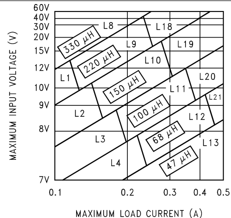
Figure 28. LM2594xx 5-V
