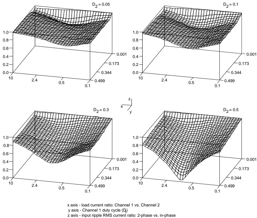
Figure 32. Input Ripple RMS Current Ratio: 2-phase vs. In-phase
