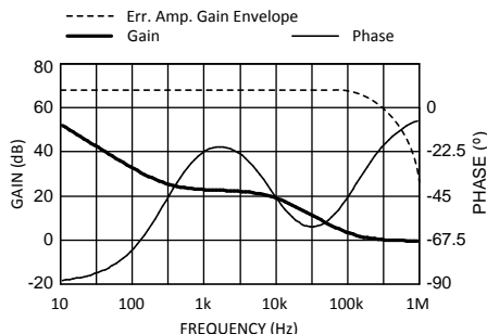
Figure 38. Example Compensation Transfer Function
