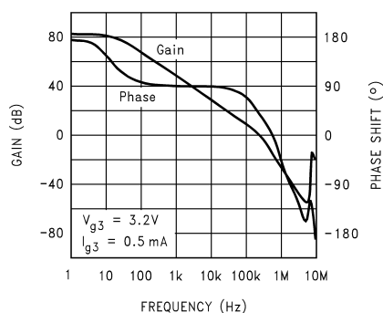
Figure 47. V_{\text{FB3-to-}V_{\text{G3}} Transfer Function (theoretical)
