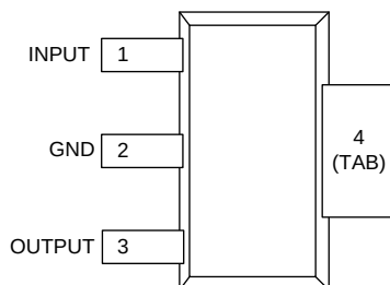
DDPAK/TO-263 Surface-Mount Package (KTT)
