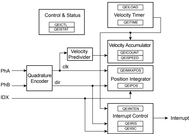
Figure 17-1. QEI Block Diagram
