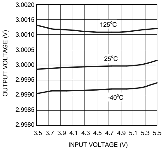
Figure 31. Line Regulation
