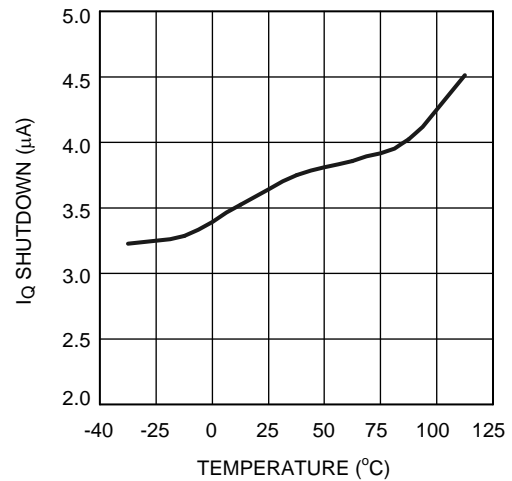
Figure 4. Shutdown I_Q vs Temperature
