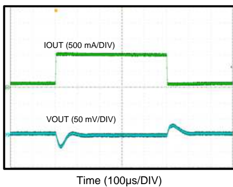
Figure 51. Output Voltage Regulation
