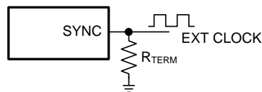
Figure 42. Frequency Synchronization
