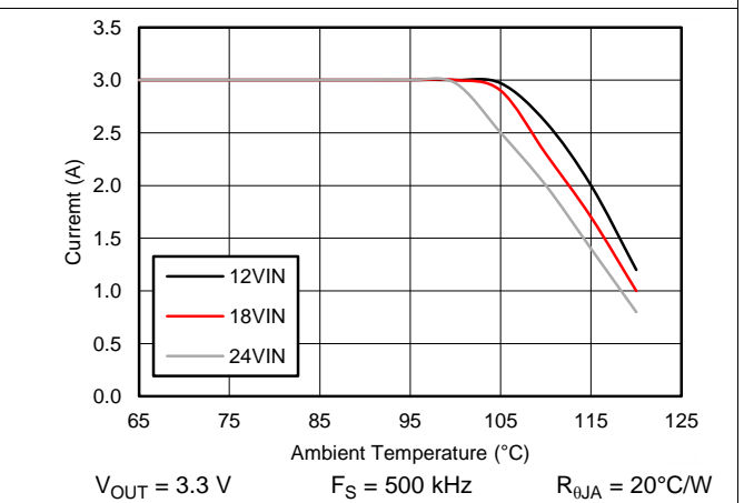
Figure 66. Derating Curve
