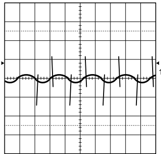
Input Voltage = 48VDC Output Current = 30 A Bandwidth Limit = 25 MHz Trace 1: Output Voltage V/div = 50 mV Horizontal Resolution = 2 \mu s/div
