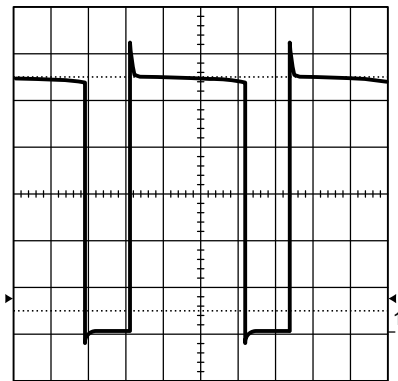
Input Voltage = 78VDC Output Current = 25 A Trace 1: Q1 Drain Voltage V/div = 20 V Horizontal Resolution = 1 \mu s/div
