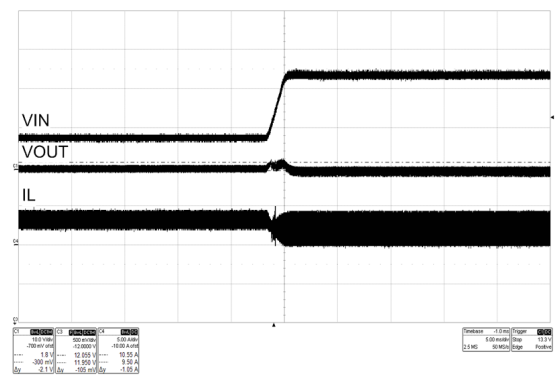
Figure 28. Line Transient Response (8 V - 24 V, I OUT = 2 A)
