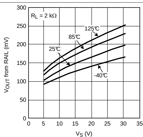
Figure 22. Positive Output Swing vs Supply Voltage
