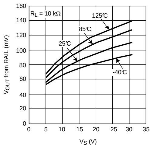
Figure 23. Positive Output Swing vs Supply Voltage
