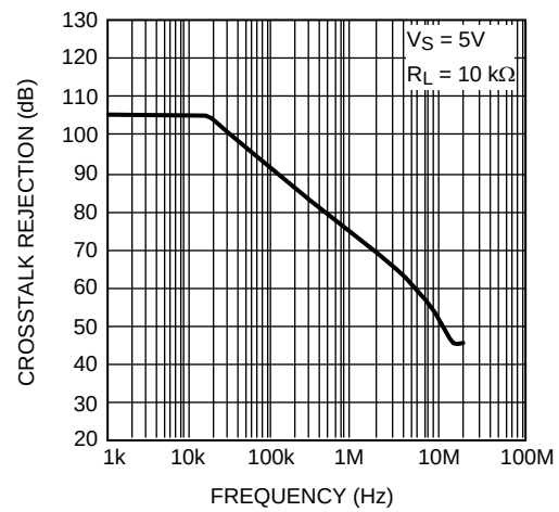
Figure 52. Crosstalk Rejection vs. Frequency
