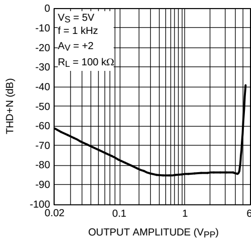
Figure 51. THD+N vs Output Amplitude
