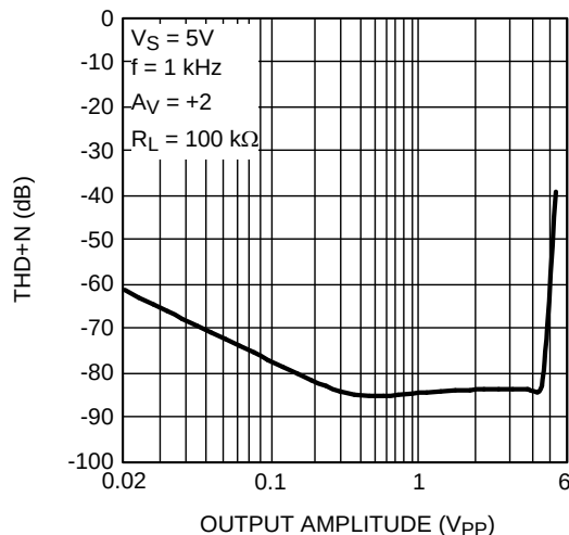
Figure 43. THD+N vs Output Amplitude ( V_{PP} )
