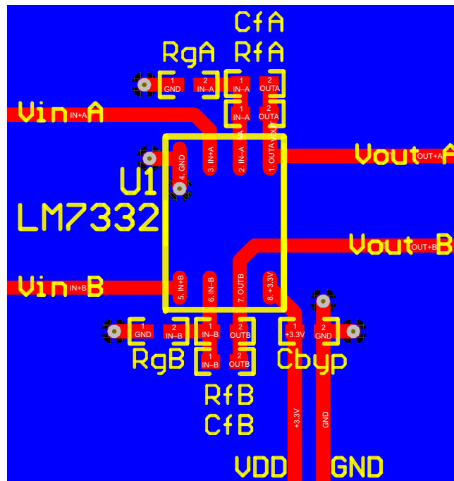
Figure 53. LM7332 Layout Example
