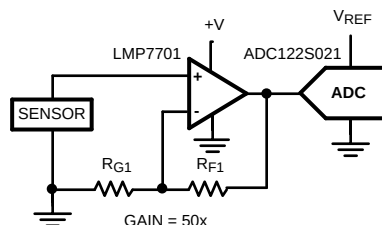
Figure 24. Sensor With DC Output and a Single-Supply Op Amp
