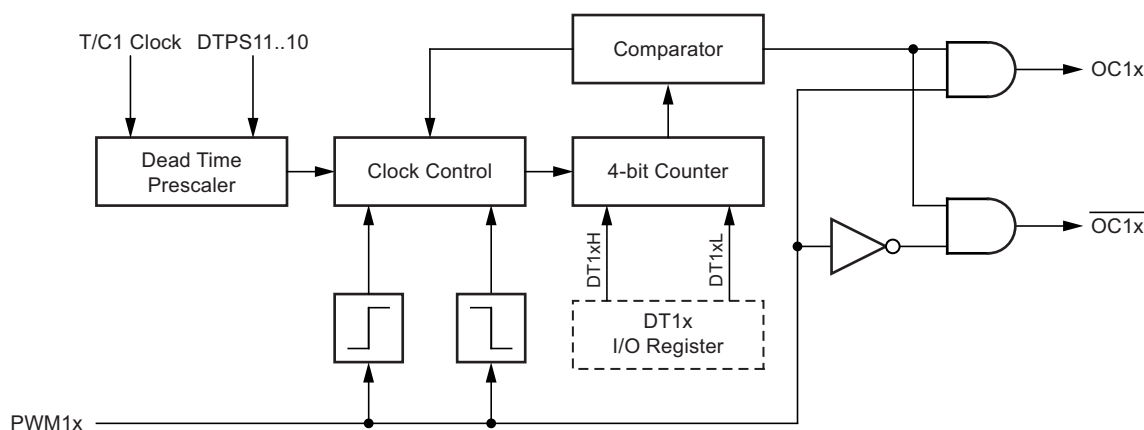
Figure 14-2. Dead Time Generator
