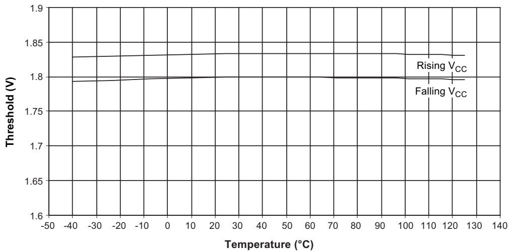
Figure 22-33. BOD Thresholds versus Temperature (BODLEVEL Is 1.8V)
