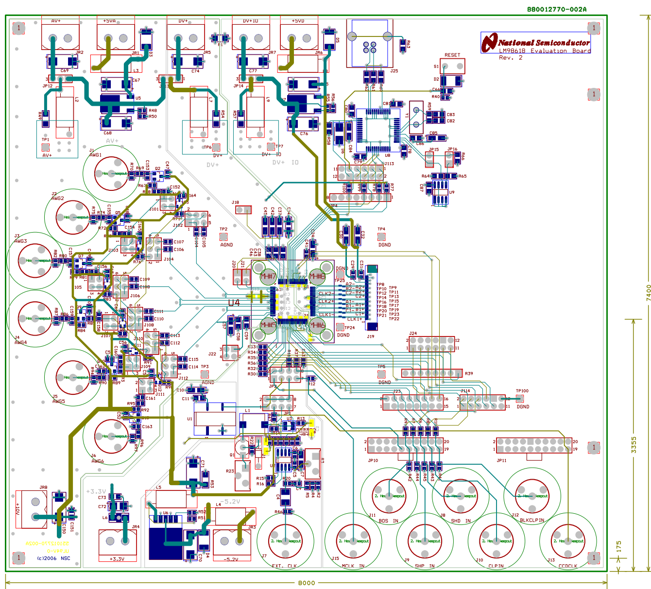
Figure 43. LM98620 Layout Example
