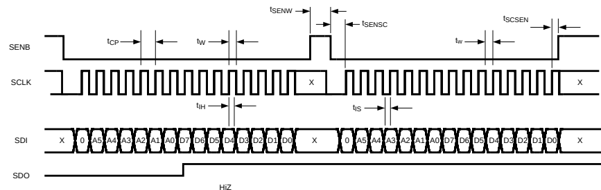
Figure 38. Serial Write
