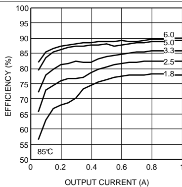
Figure 21. Efficiency 12-V Input at 85°C
