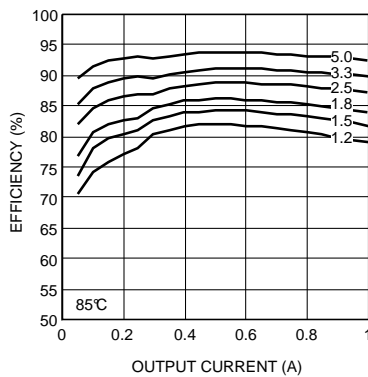
Figure 19. Efficiency 8-V Input at 85°C
