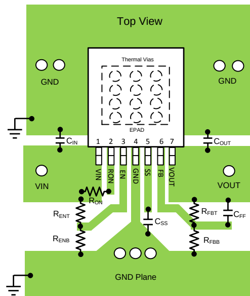
Figure 43. PCB Layout Guide
