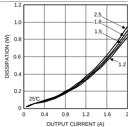
Figure 4. Dissipation 5-V Input at 25°C
