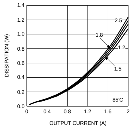
Figure 16. Dissipation 5-V Input at 85°C
