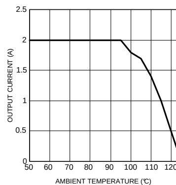
Figure 40. Thermal Derating Curve
