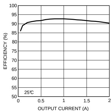
Figure 39. Efficiency
