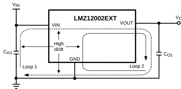
Figure 42. Critical Current Loops to Minimize
