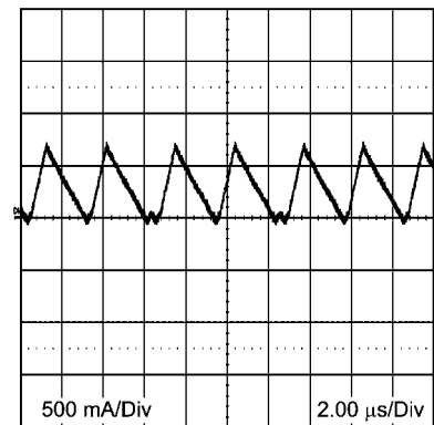
Transition Mode Operation V_{IN} = 24V, V_O = 3.3V, I_O = 0.35A \quad 2 \mu\text{sec/div}
