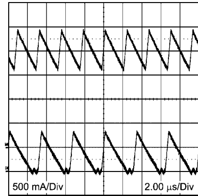
CCM and DCM Operating Modes V_{IN} = 24V, V_O = 3.3V, I_O = 2A/0.32A \quad 2 \mu\text{sec/div}
