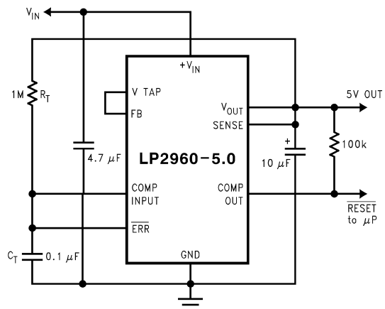
Figure 9. 5V Regulator with Timed Power-On Reset
