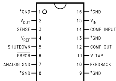
Figure 1. Top View 16-Pin Surface Mount Package
