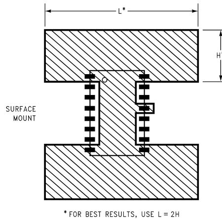
Figure 4. Heat Sink Foil Patterns
