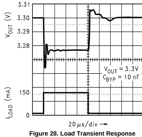
Figure 28. Load Transient Response
