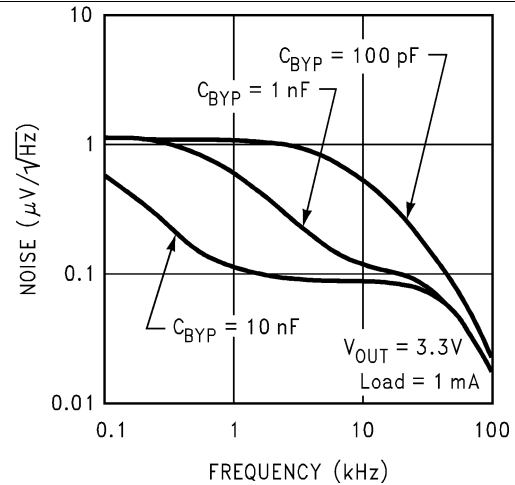
Figure 14. Output Noise Density
