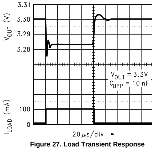
Figure 27. Load Transient Response
